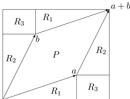
Figure 2. The area of the parallelotope determined by a and b .
